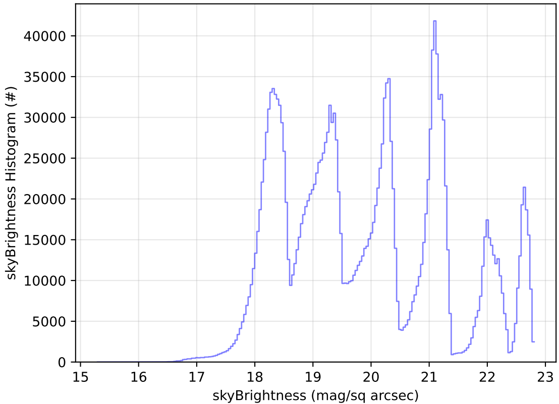
ddf_acor_sf10_lsf15_lsr10_v3.4_10yrs WFD all bands: skyBrightness Histogram
