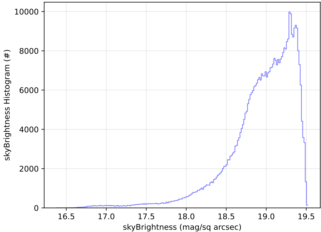
ddf_acor_sf10_lsf15_lsr10_v3.4_10yrs All sky z band: skyBrightness Histogram
