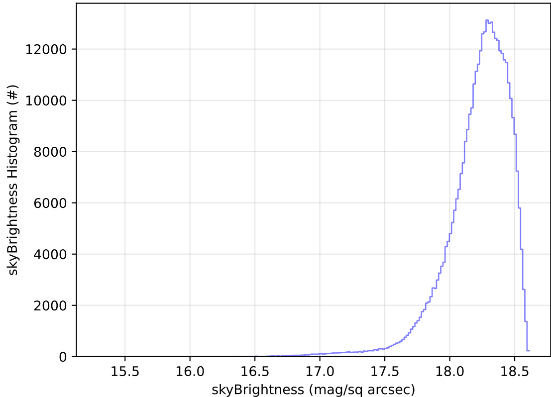
ddf_acor_sf10_lsf15_lsr10_v3.4_10yrs All sky y band: skyBrightness Histogram
