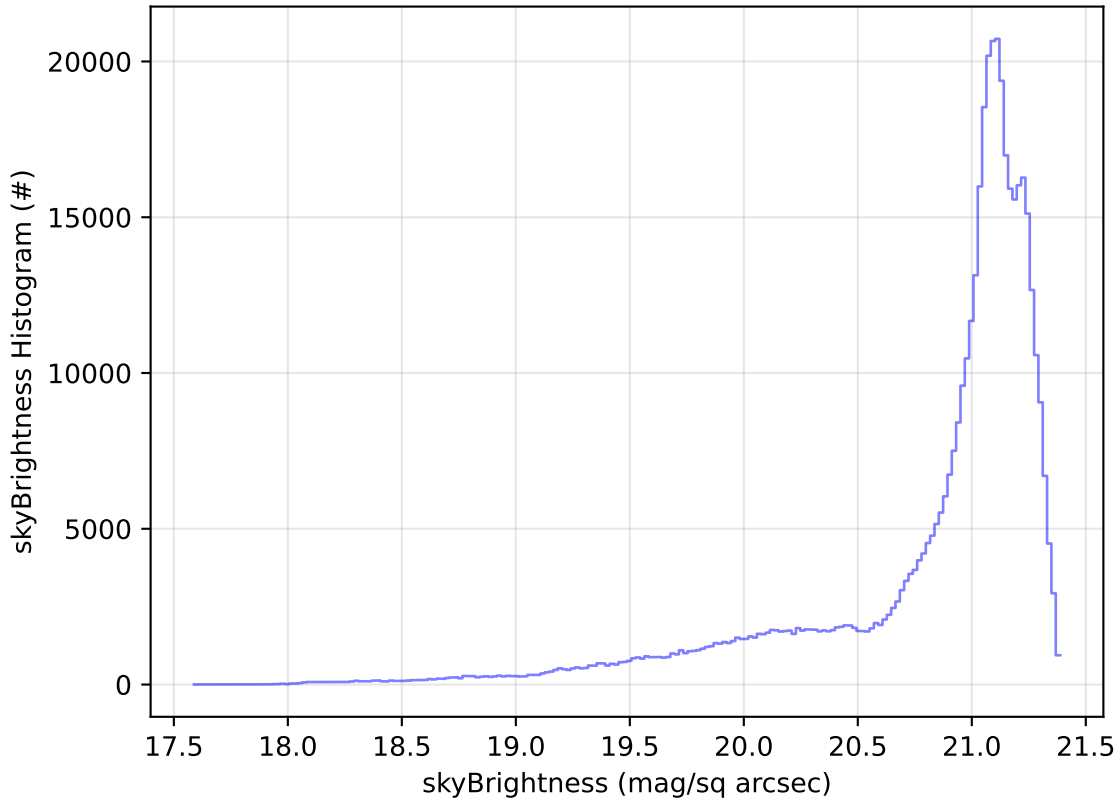
ddf_acor_sf10_lsf15_lsr10_v3.4_10yrs All sky r band: skyBrightness Histogram
