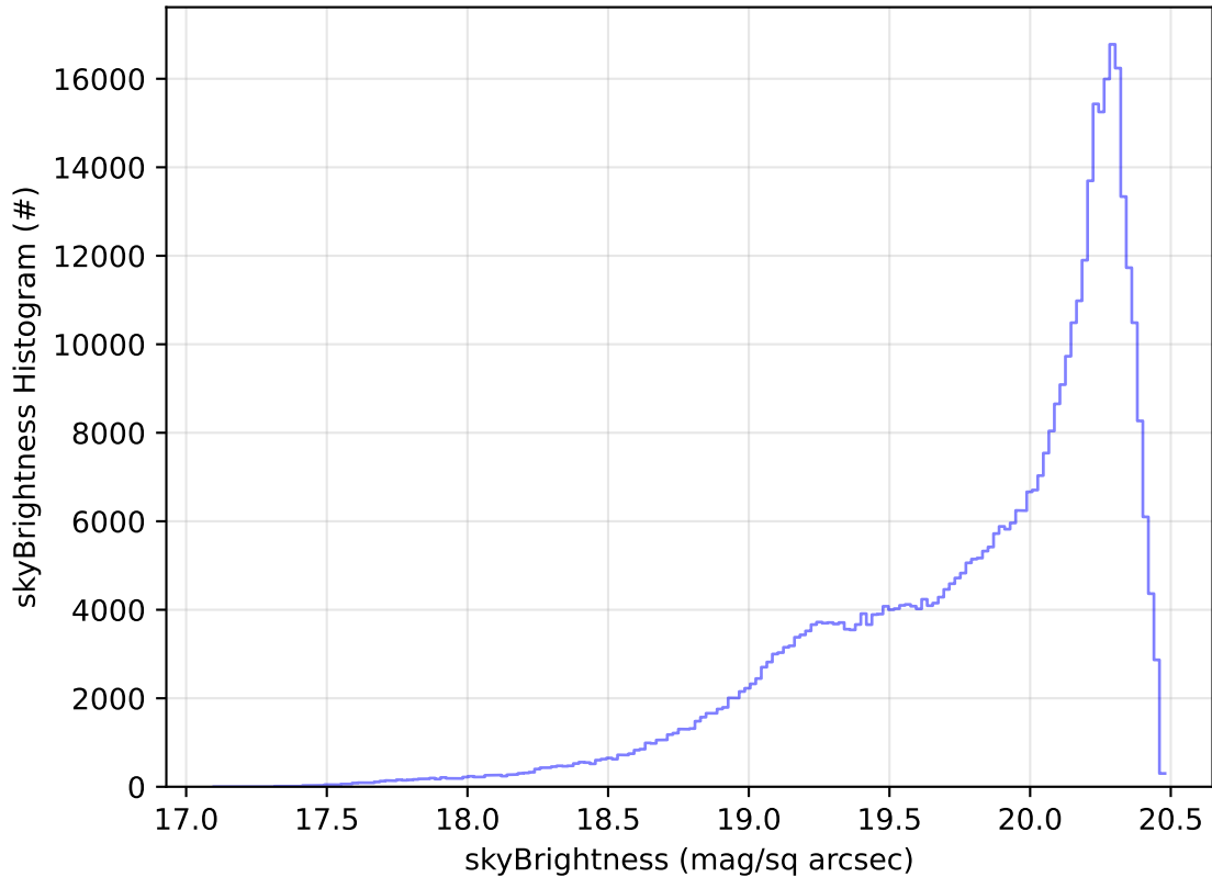
ddf_acor_sf10_lsf15_lsr10_v3.4_10yrs All sky i band: skyBrightness Histogram
