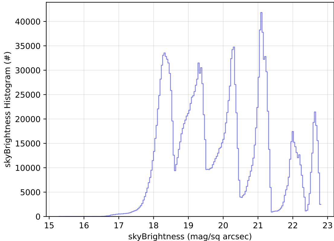
ddf_acor_sf10_lsf15_lsr10_v3.4_10yrs All sky all bands: skyBrightness Histogram
