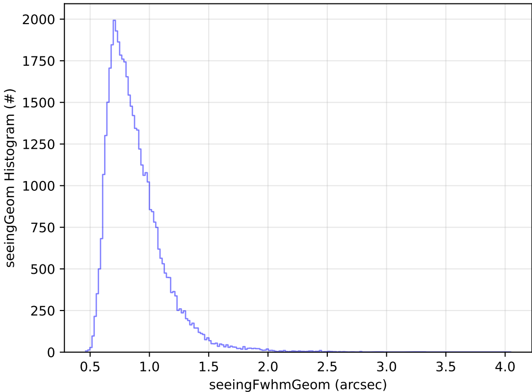
ddf_acor_sf10_lsf15_lsr10_v3.4_10yrs Yr 1 z band: seeingGeom Histogram
