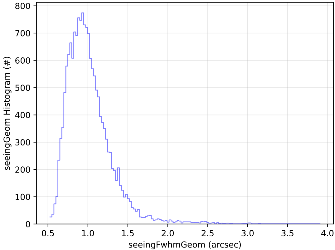
ddf_acor_sf10_lsf15_lsr10_v3.4_10yrs Yr 1 u band: seeingGeom Histogram
