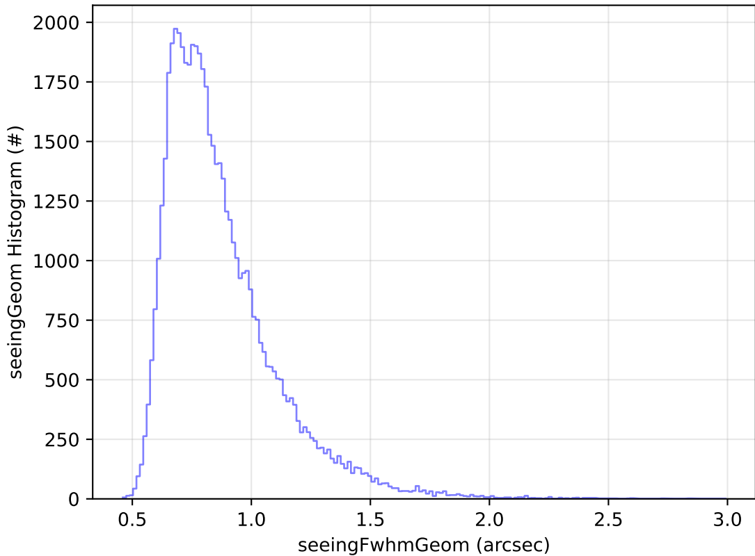
ddf_acor_sf10_lsf15_lsr10_v3.4_10yrs Yr 1 i band: seeingGeom Histogram
