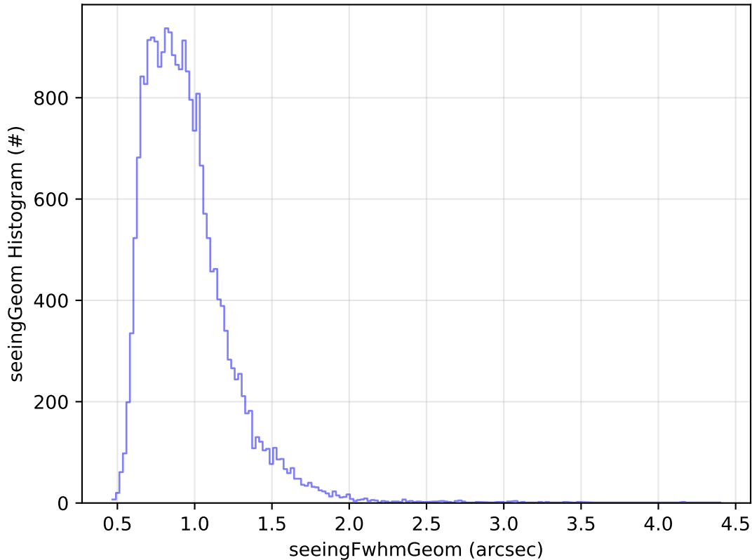
ddf_acor_sf10_lsf15_lsr10_v3.4_10yrs Yr 1 g band: seeingGeom Histogram
