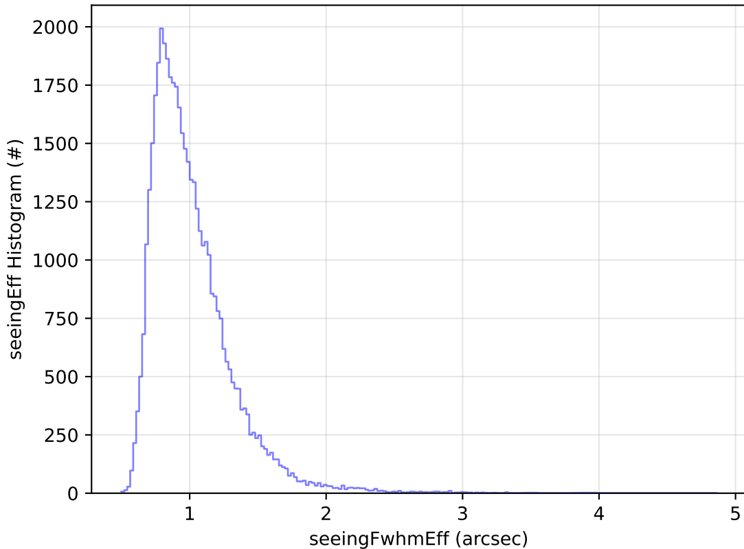
ddf_acor_sf10_lsf15_lsr10_v3.4_10yrs Yr 1 z band: seeingEff Histogram
