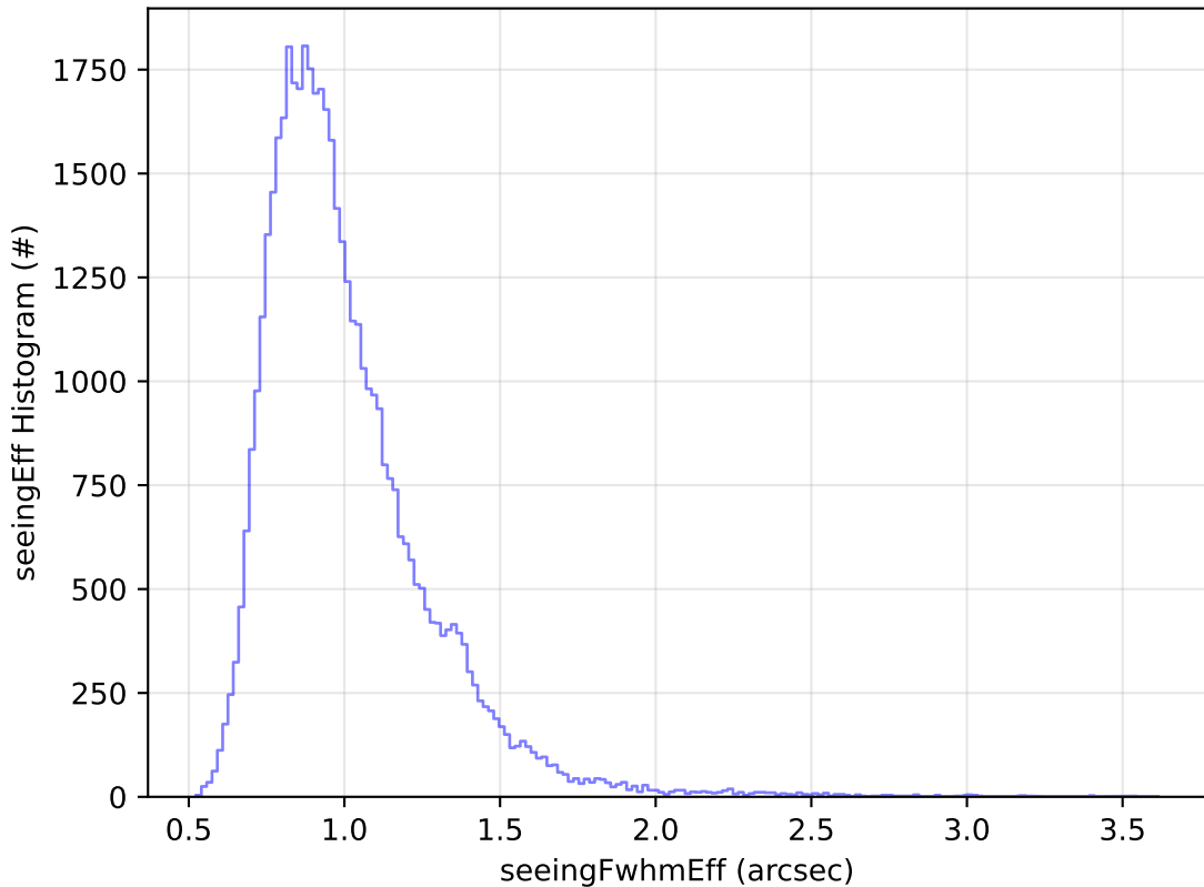
ddf_acor_sf10_lsf15_lsr10_v3.4_10yrs Yr 1 y band: seeingEff Histogram
