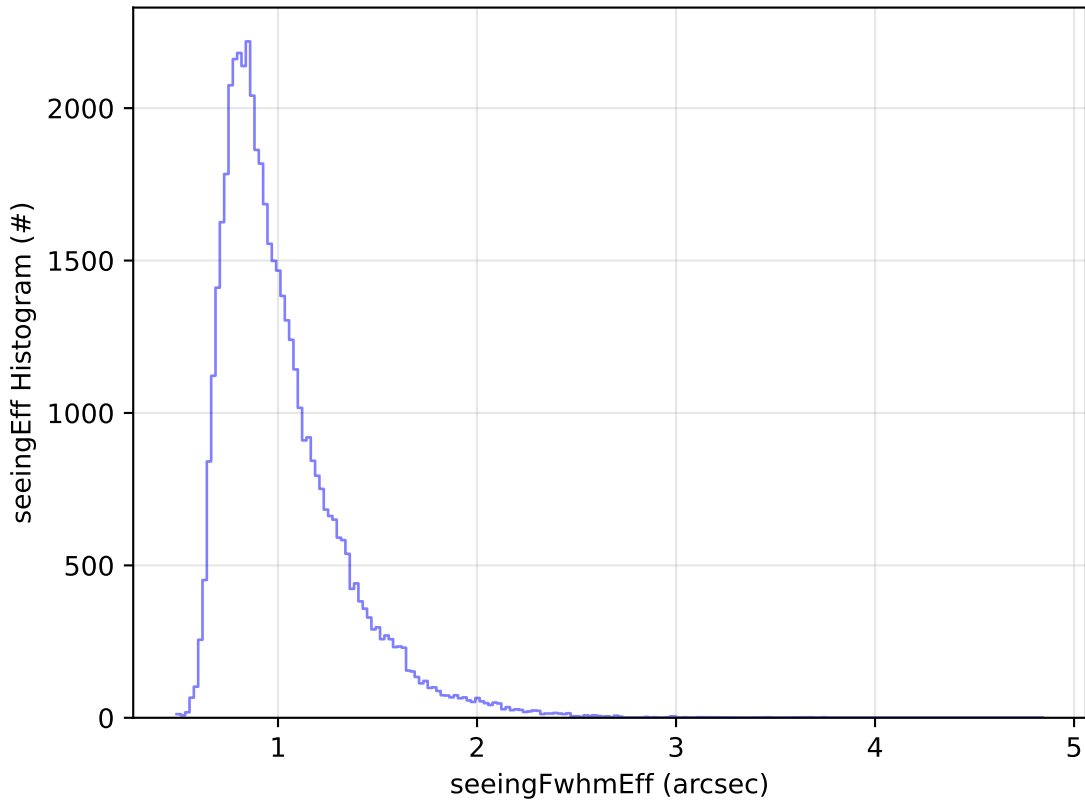
ddf_acor_sf10_lsf15_lsr10_v3.4_10yrs Yr 1 r band: seeingEff Histogram
