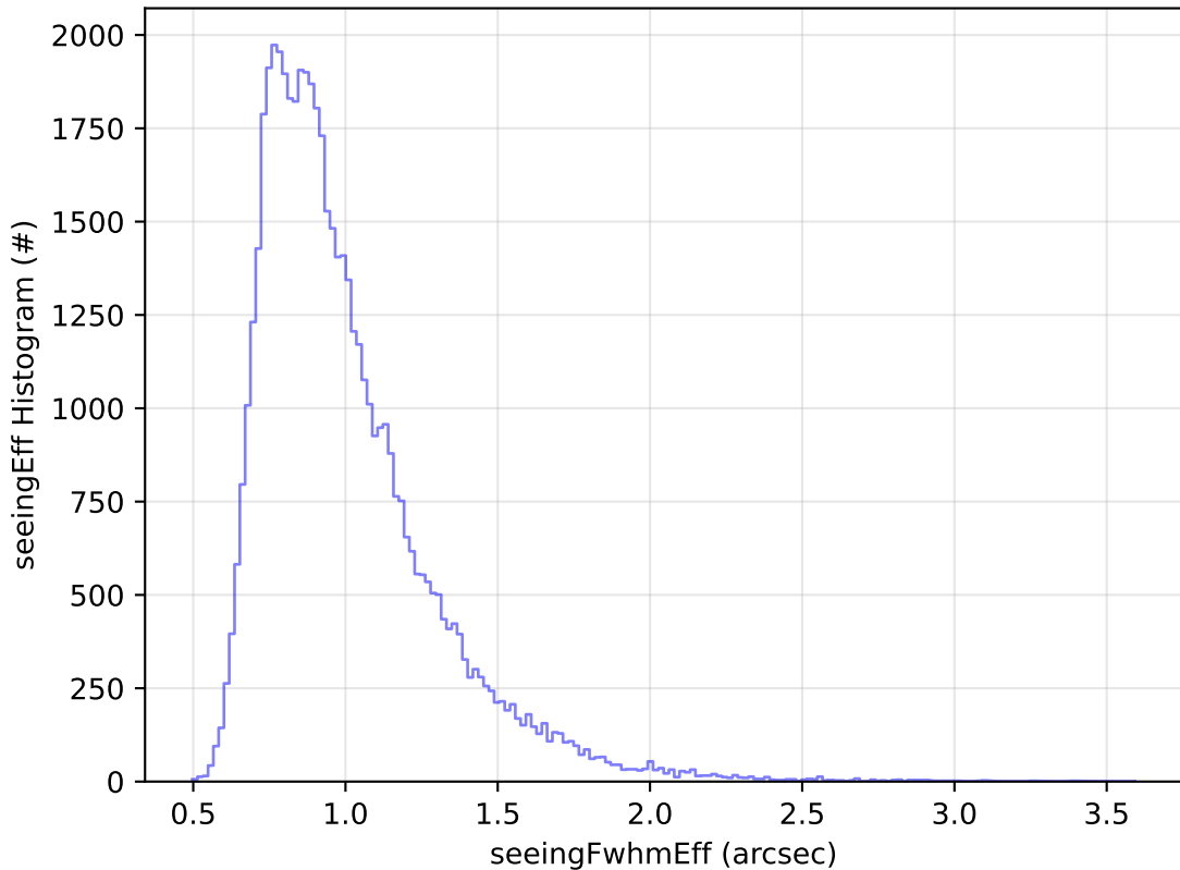
ddf_acor_sf10_lsf15_lsr10_v3.4_10yrs Yr 1 i band: seeingEff Histogram
