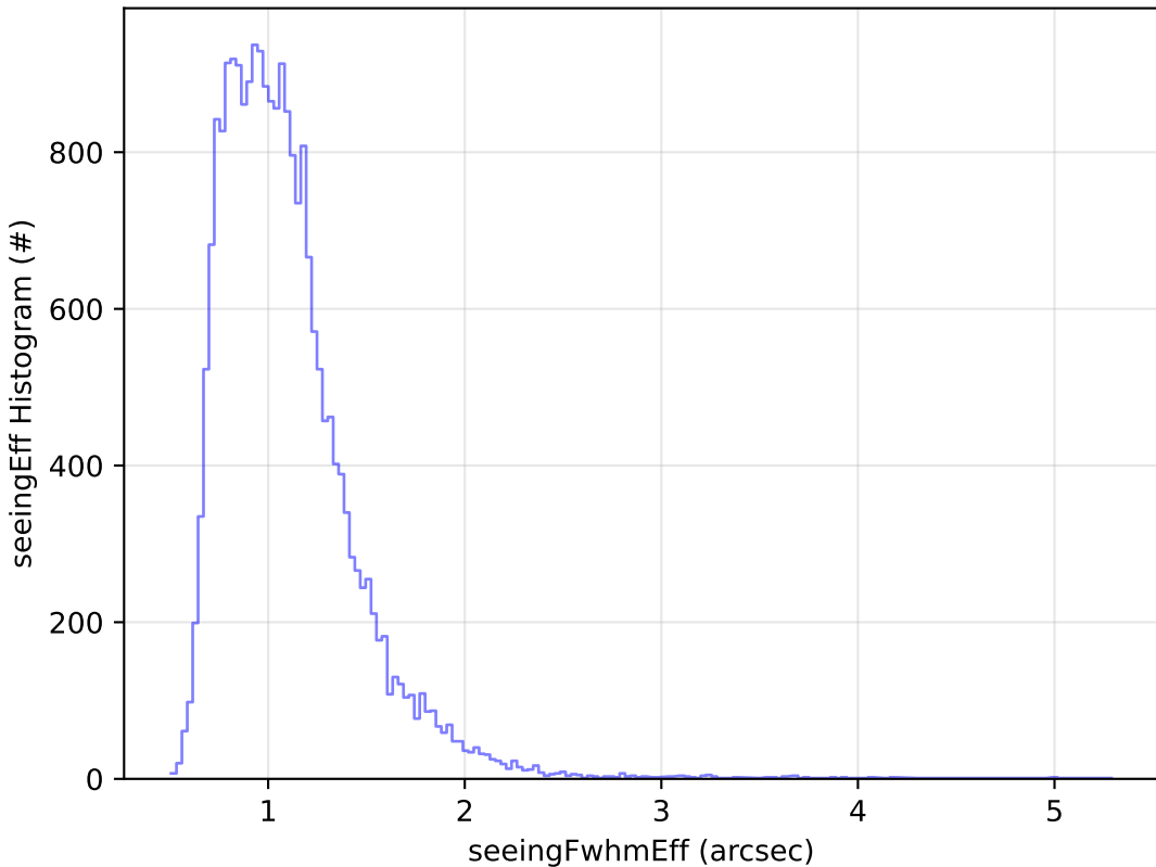
ddf_acor_sf10_lsf15_lsr10_v3.4_10yrs Yr 1 g band: seeingEff Histogram
