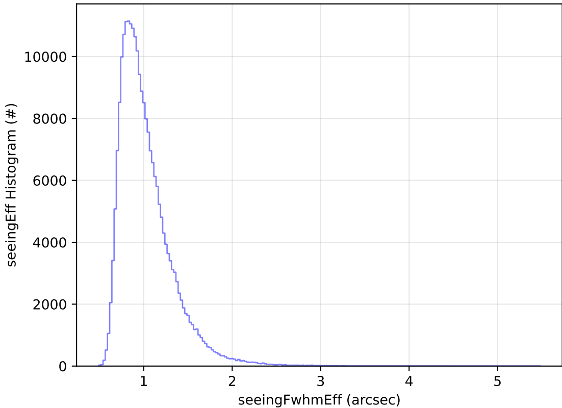
ddf_acor_sf10_Isf15_Isr10_v3.4_10yrs Yr 1 all bands: seeingEff Histogram
