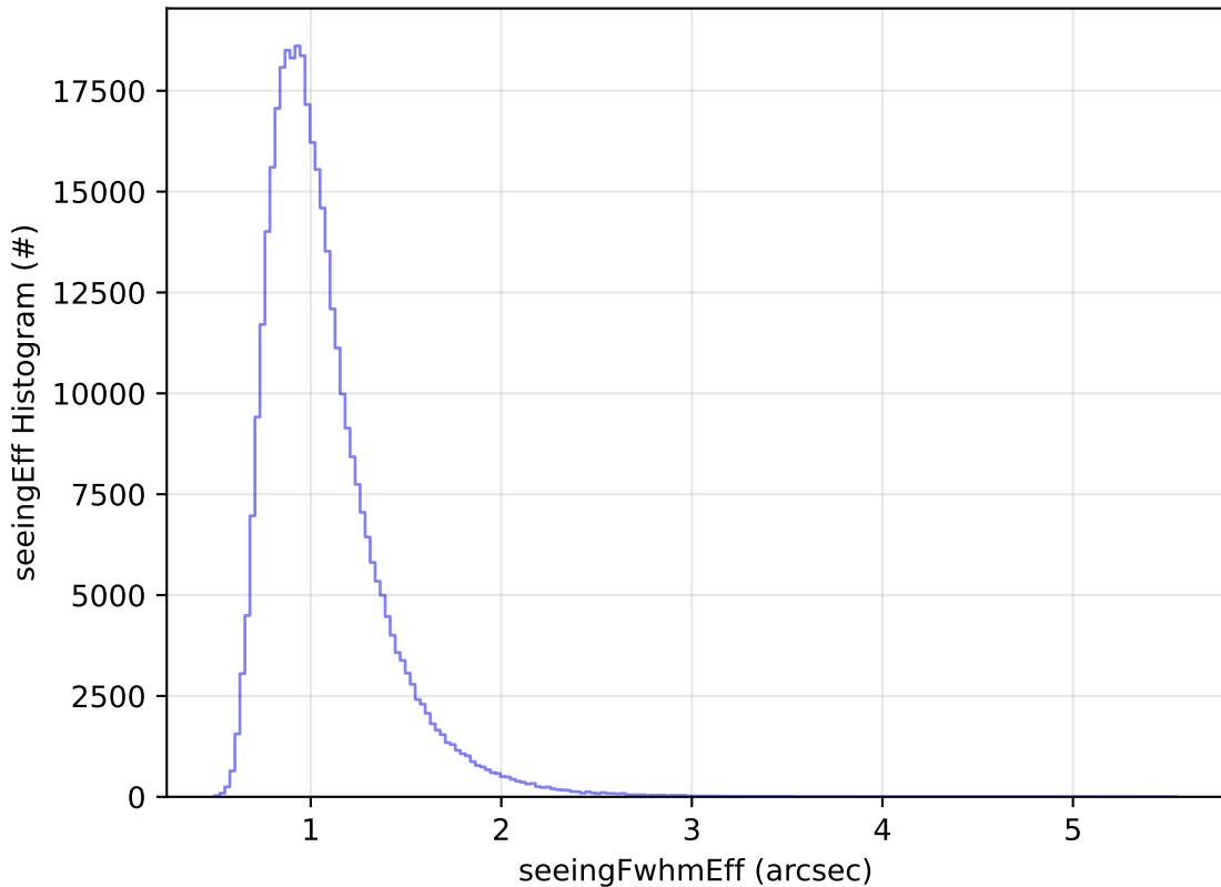
ddf_acor_sf10_lsf15_lsr10_v3.4_10yrs WFD y band: seeingEff Histogram
