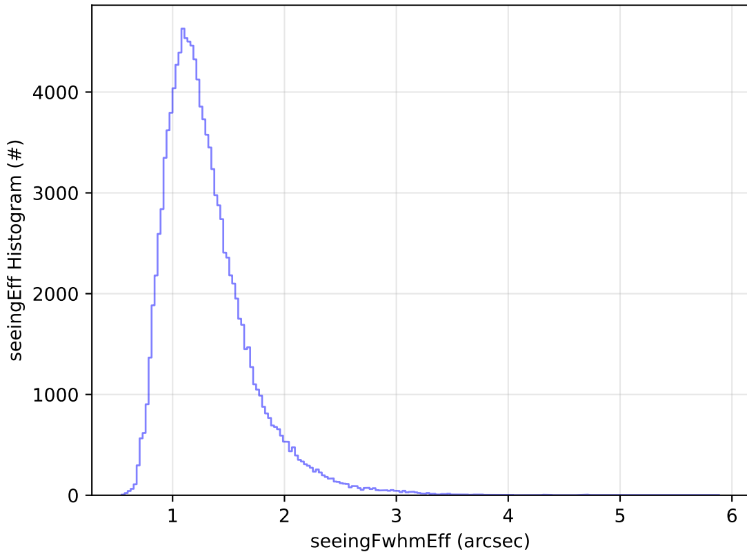
ddf_acor_sf10_lsf15_lsr10_v3.4_10yrs WFD u band: seeingEff Histogram
