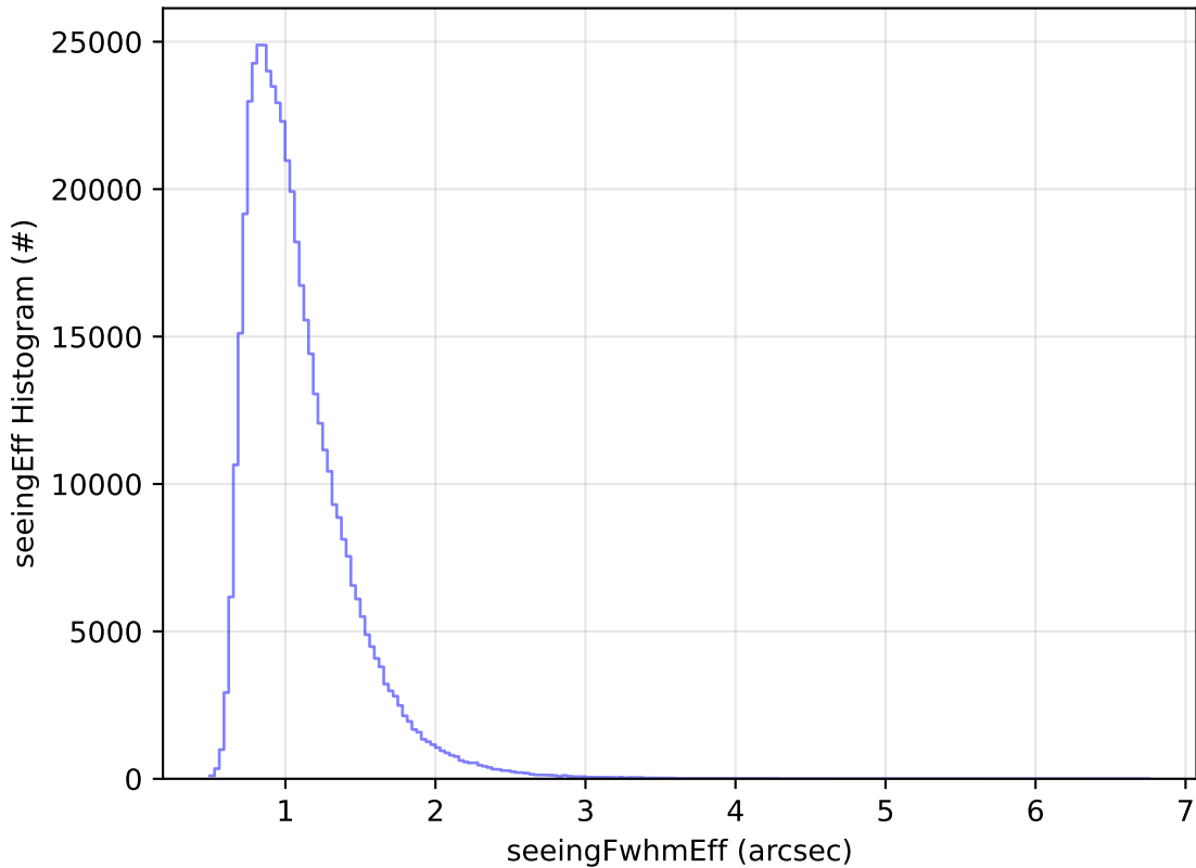
ddf_acor_sf10_lsf15_lsr10_v3.4_10yrs WFD i band: seeingEff Histogram
