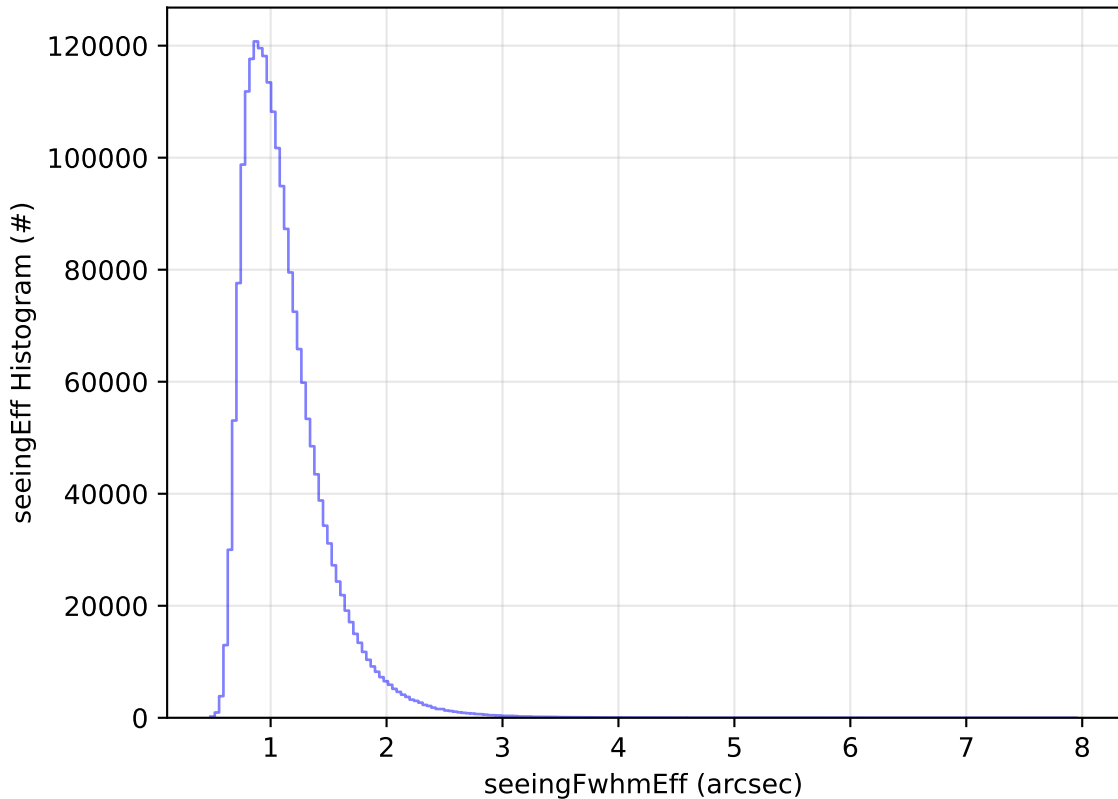
ddf_acor_sf10_lsf15_lsr10_v3.4_10yrs WFD all bands: seeingEff Histogram
