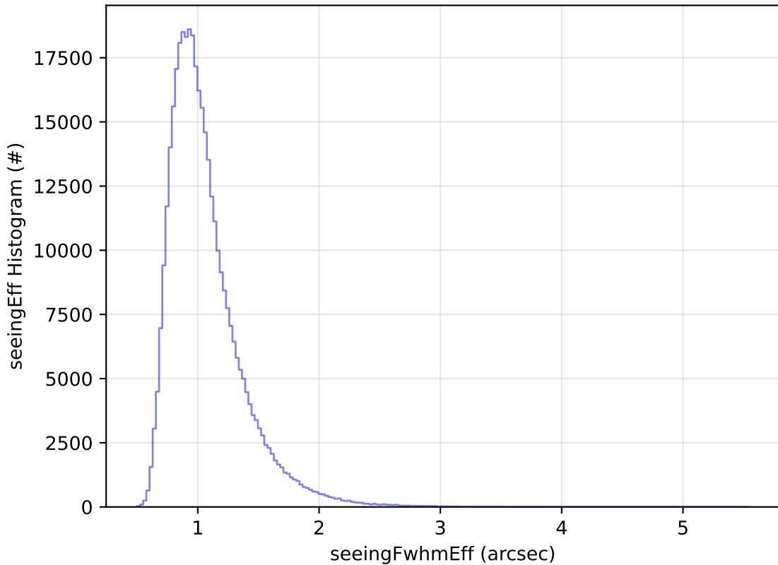
ddf_acor_sf10_lsf15_lsr10_v3.4_10yrs All sky y band: seeingEff Histogram
