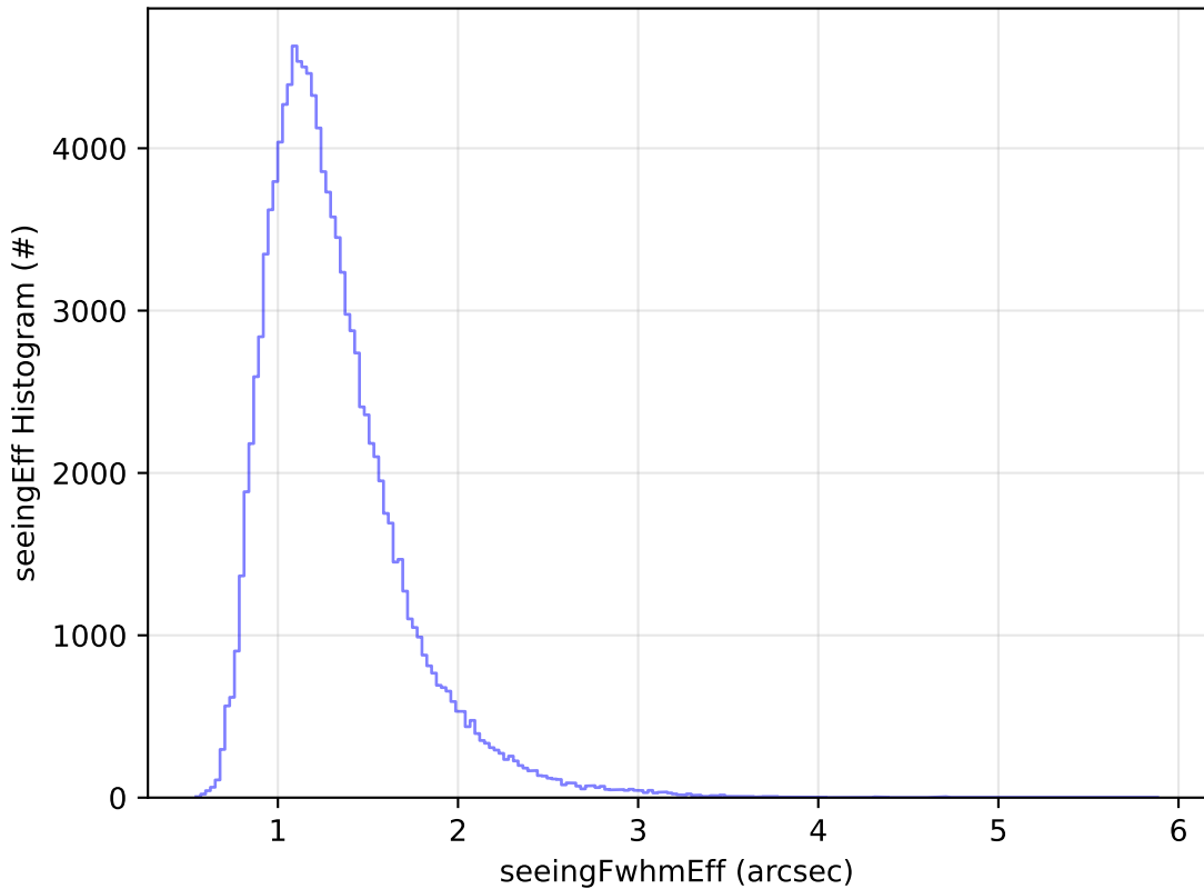
ddf_acor_sf10_ls15_lsr10_v3.4_10yrs All sky u band: seeingEff Histogram
