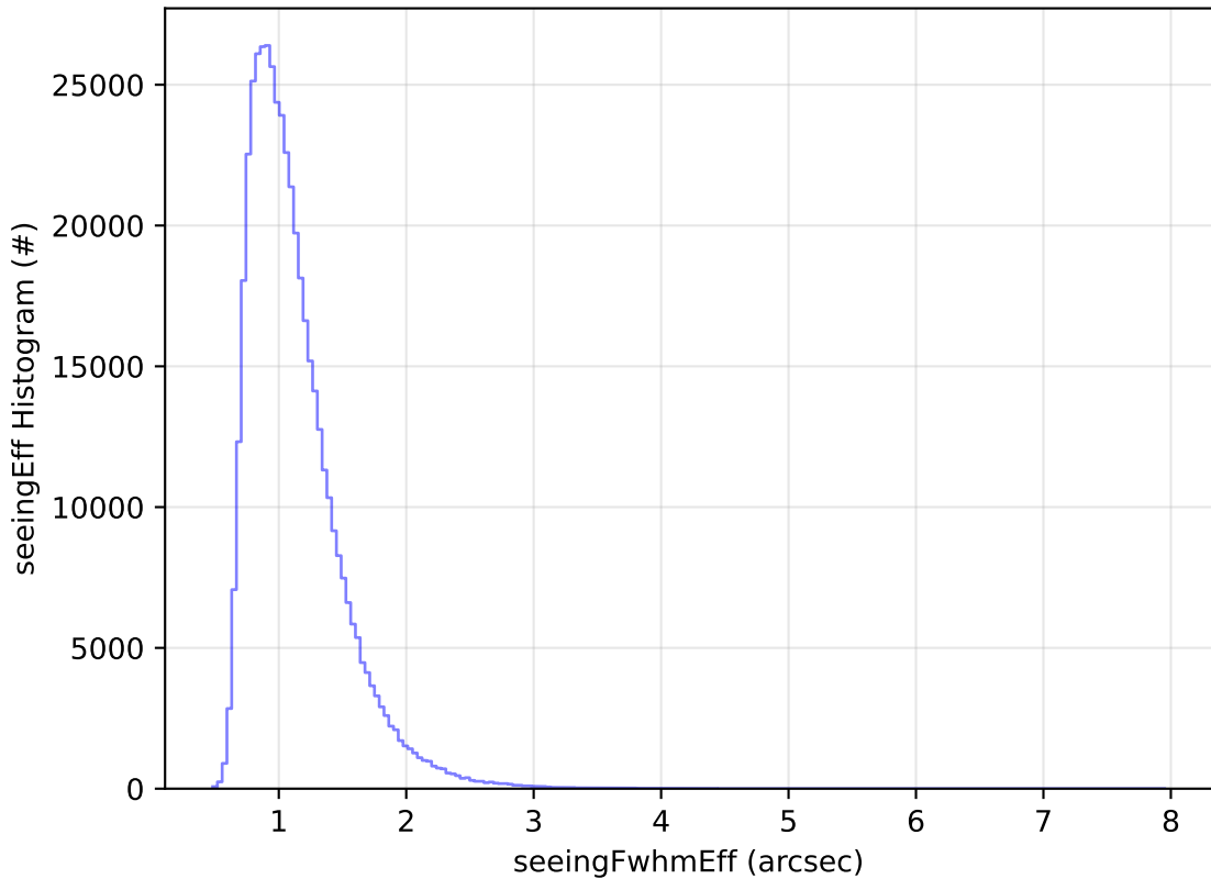
ddf_acor_sf10_lsf15_lsr10_v3.4_10yrs All sky r band: seeingEff Histogram
