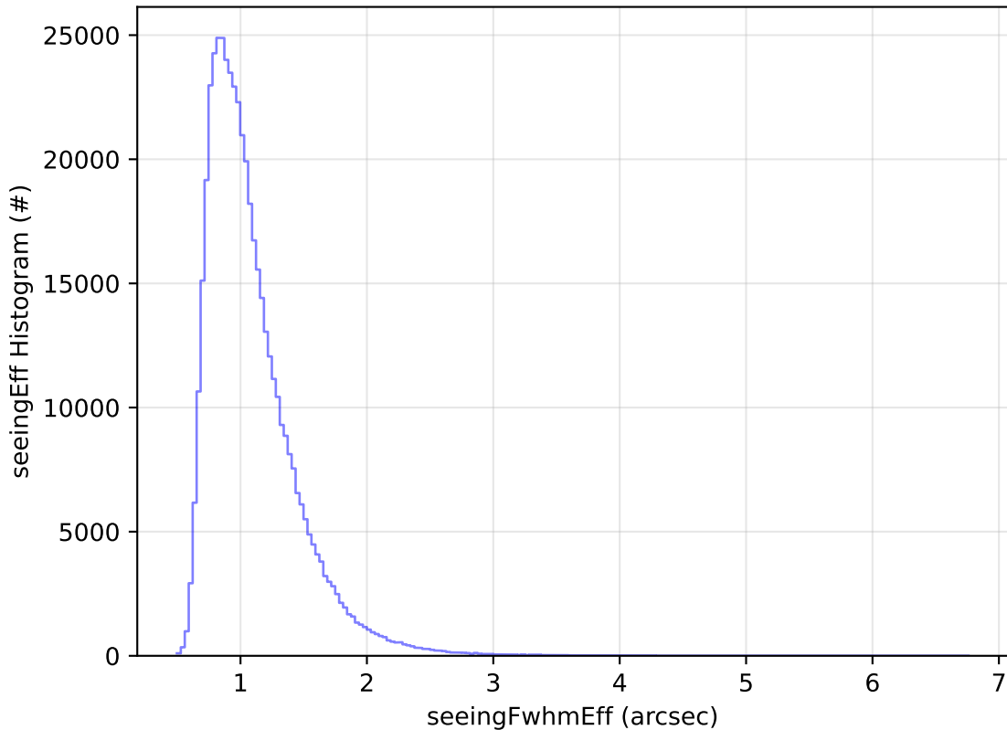
ddf_acor_sf10_lsf15_lsr10_v3.4_10yrs All sky i band: seeingEff Histogram
