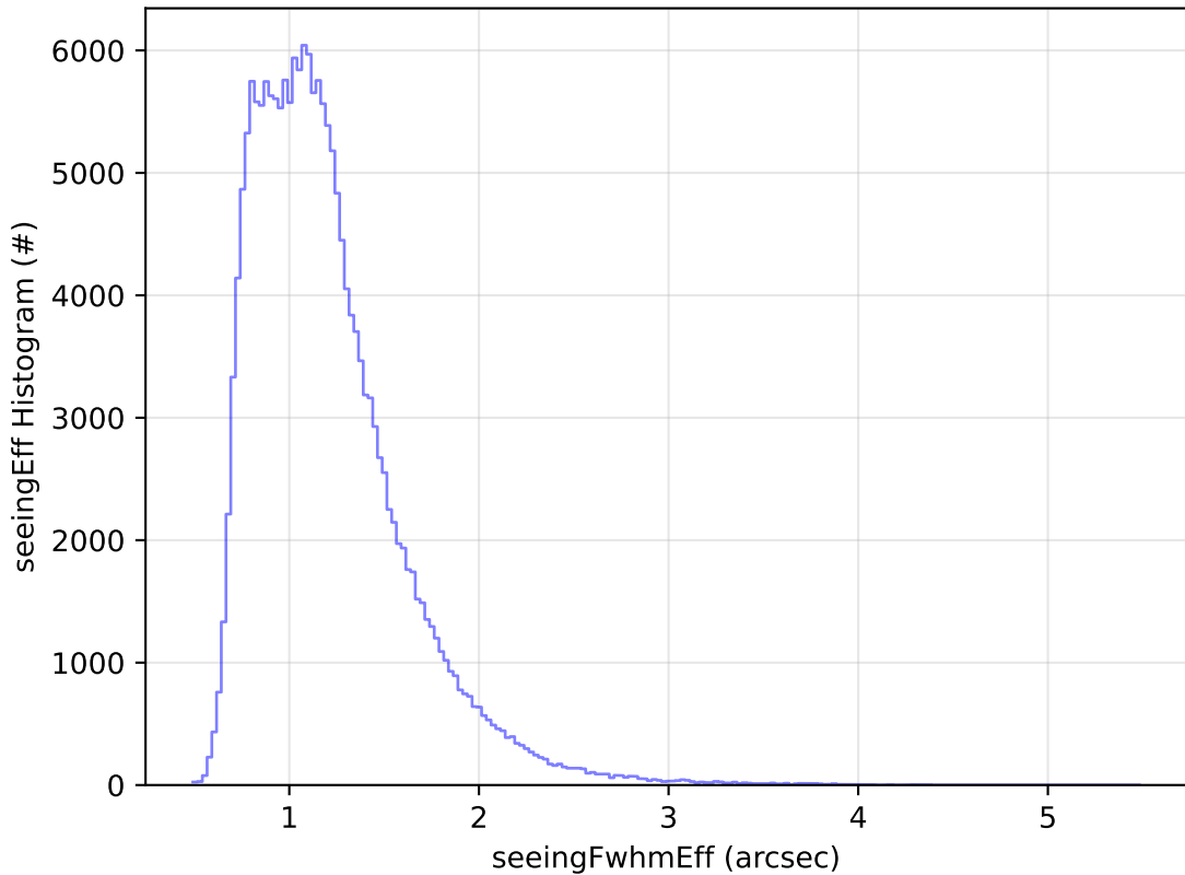
ddf_acor_sf10_ls15_lsr10_v3.4_10yrs All sky g band: seeingEff Histogram
