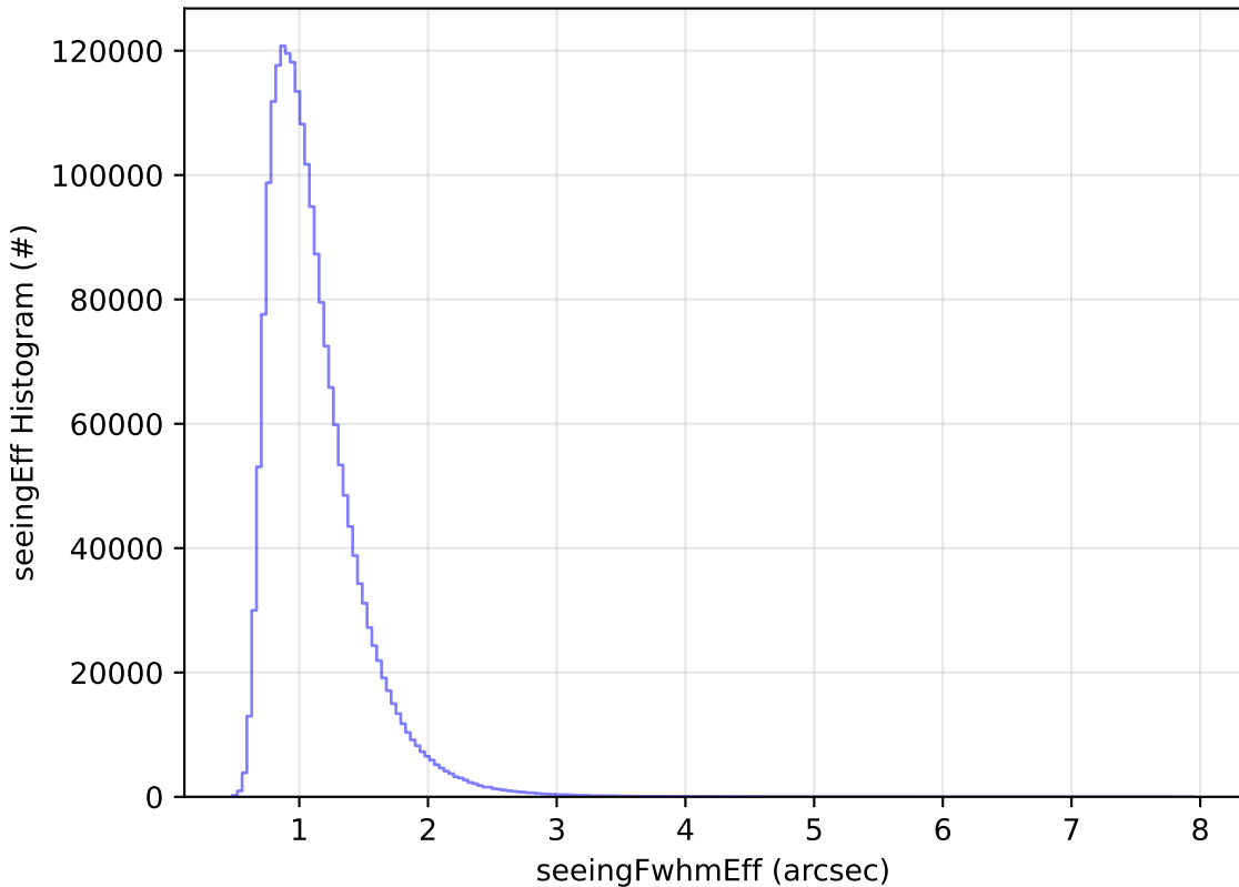
ddf_acor_sf10_lsf15_lsr10_v3.4_10yrs All sky all bands: seeingEff Histogram
