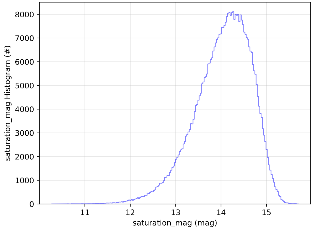
ddf_acor_sf10_lsf15_lsr10_v3.4_10yrs WFD z band: saturation_mag Histogram
