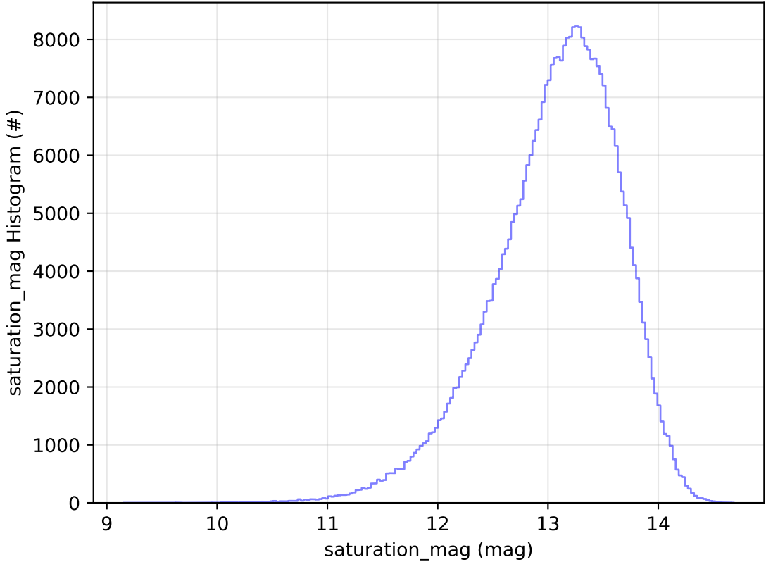
ddf_acor_sf10_lsf15_lsr10_v3.4_10yrs WFD y band: saturation_mag Histogram
