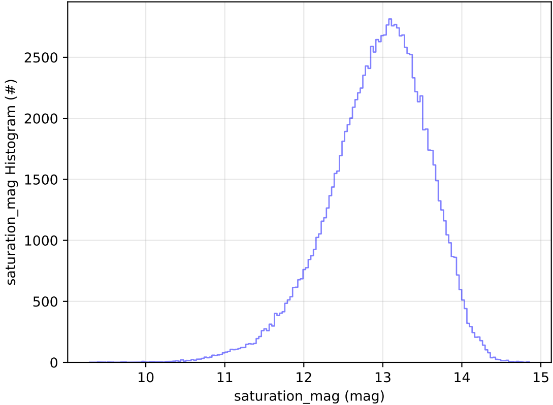
ddf_acor_sf10_lsf15_lsr10_v3.4_10yrs WFD u band: saturation_mag Histogram
