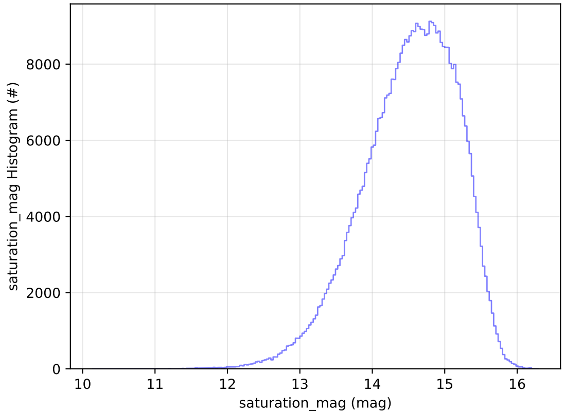
ddf_acor_sf10_lsf15_lsr10_v3.4_10yrs WFD r band: saturation_mag Histogram
