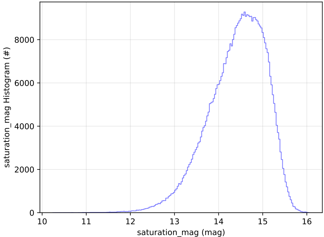
ddf_acor_sf10_lsf15_lsr10_v3.4_10yrs WFD i band: saturation_mag Histogram
