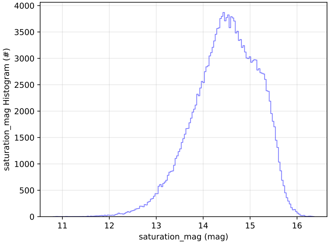
ddf_acor_sf10_lsf15_lsr10_v3.4_10yrs WFD g band: saturation_mag Histogram
