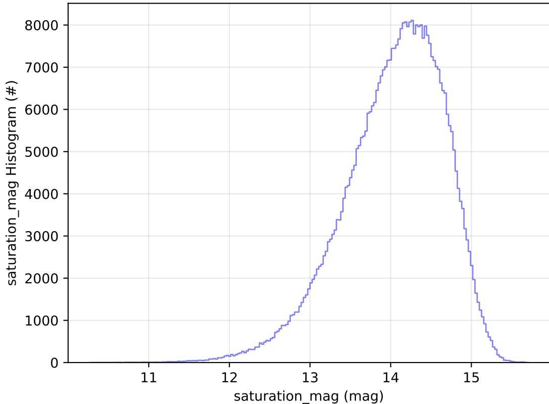
ddf_acor_sf10_lsf15_lsr10_v3.4_10yrs All sky z band: saturation_mag Histogram
