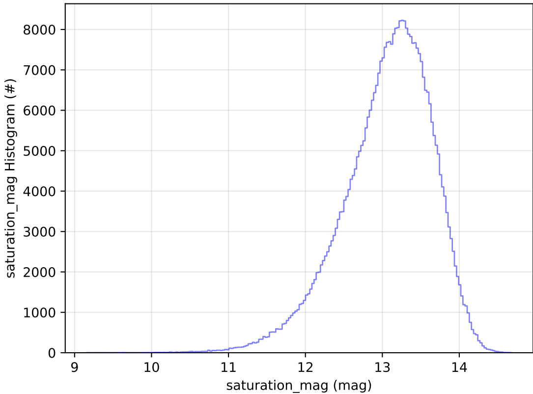
ddf_acor_sf10_lsf15_lsr10_v3.4_10yrs All sky y band: saturation_mag Histogram
