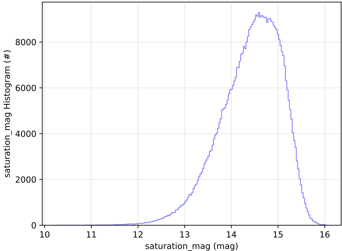
ddf_acor_sf10_lsf15_lsr10_v3.4_10yrs All sky i band: saturation_mag Histogram
