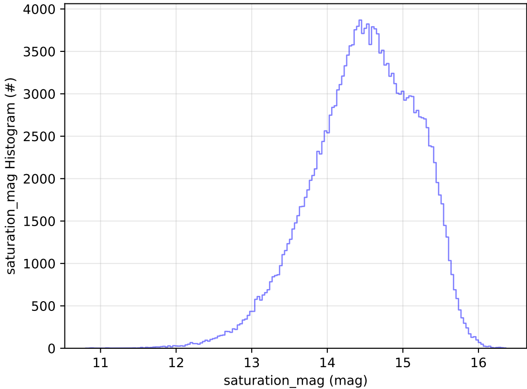
ddf_acor_sf10_lsf15_lsr10_v3.4_10yrs All sky g band: saturation_mag Histogram
