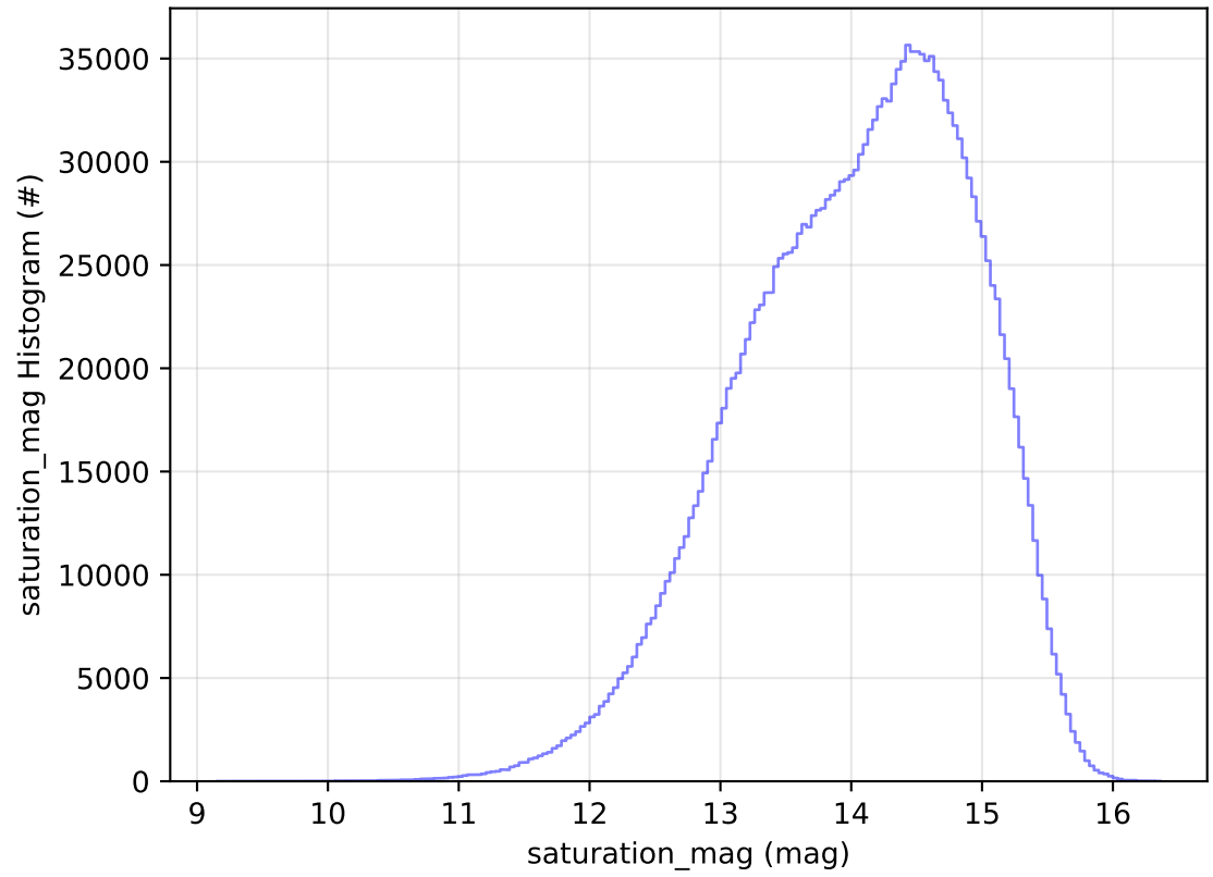
ddf_acor_sf10_lsf15_lsr10_v3.4_10yrs All sky all bands: saturation_mag Histogram
