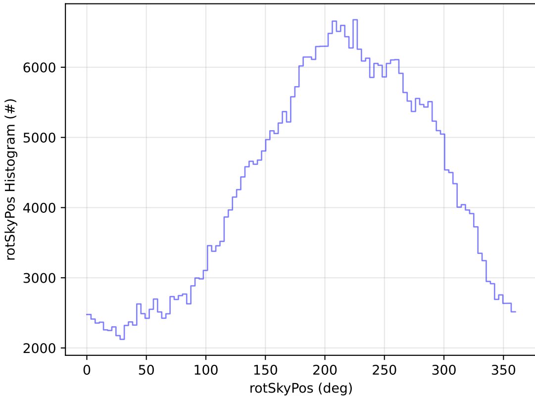
ddf_acor_sf10_lsf15_lsr10_v3.4_10yrs WFD z band: rotSkyPos Histogram
