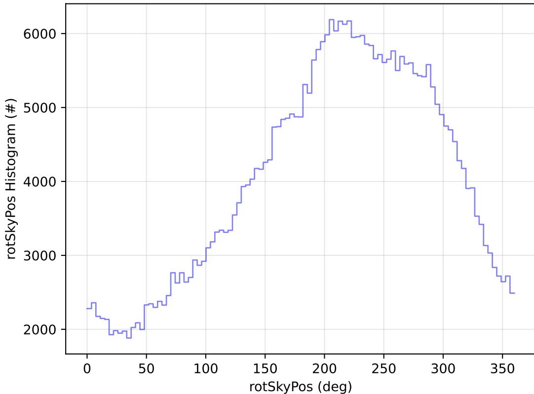
ddf_acor_sf10_lsf15_lsr10_v3.4_10yrs WFD y band: rotSkyPos Histogram
