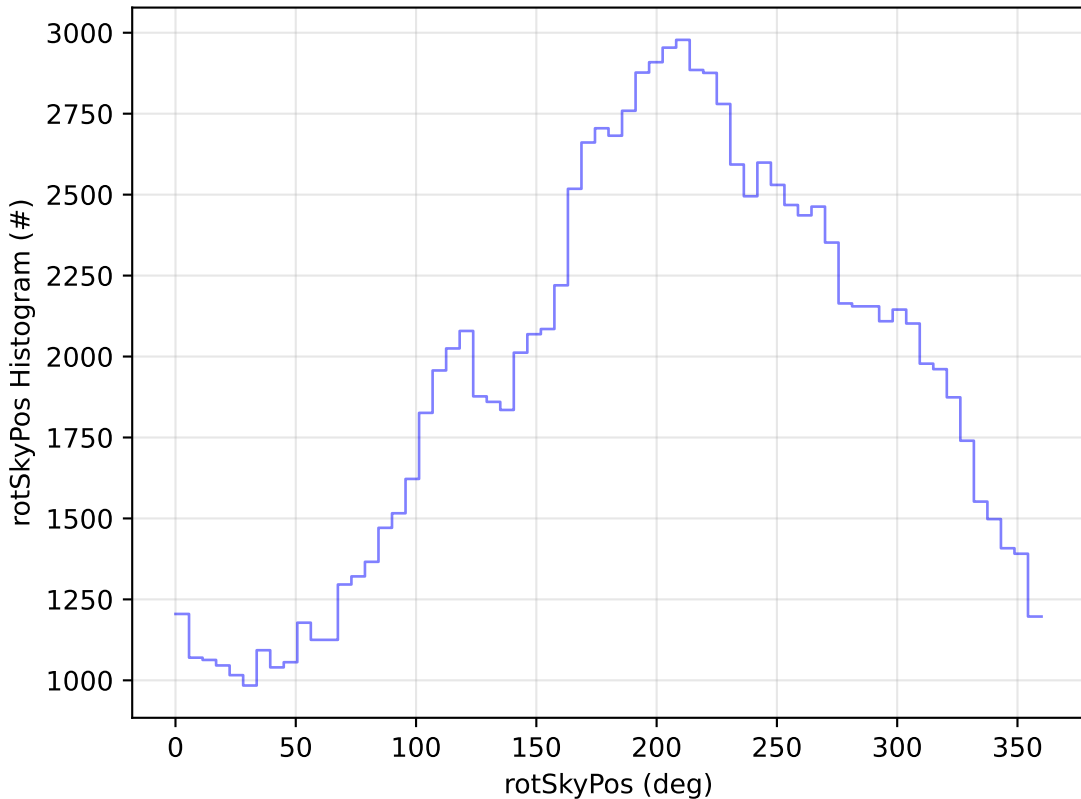
ddf_acor_sf10_lsf15_lsr10_v3.4_10yrs WFD u band: rotSkyPos Histogram
