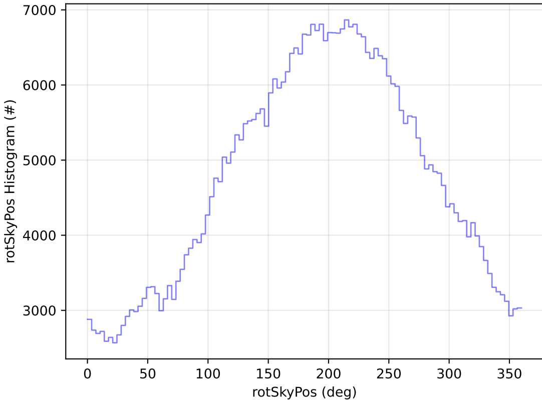
ddf_acor_sf10_lsf15_lsr10_v3.4_10yrs WFD r band: rotSkyPos Histogram
