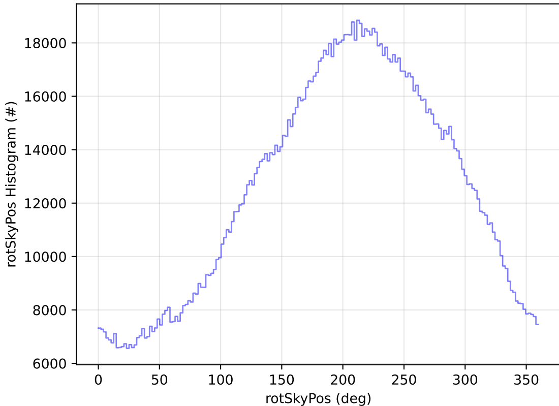
ddf_acor_sf10_lsf15_lsr10_v3.4_10yrs WFD all bands: rotSkyPos Histogram
