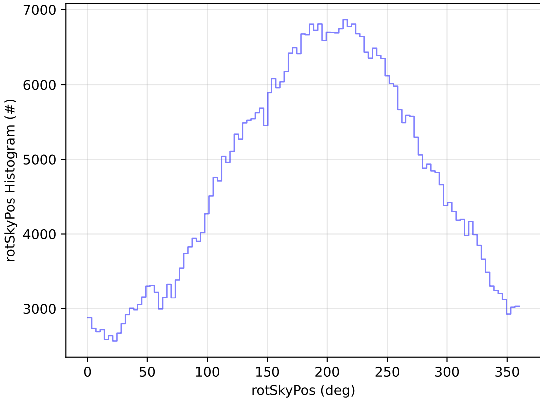
ddf_acor_sf10_ls15_lsr10_v3.4_10yrs All sky r band: rotSkyPos Histogram
