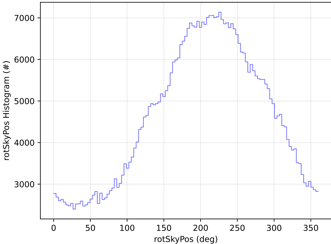
ddf_acor_sf10_ls15_lsr10_v3.4_10yrs All sky i band: rotSkyPos Histogram
