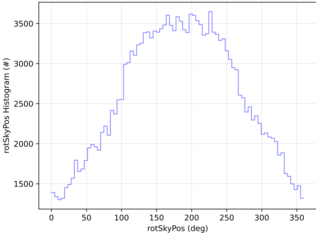
ddf_acor_sf10_lsf15_lsr10_v3.4_10yrs All sky g band: rotSkyPos Histogram
