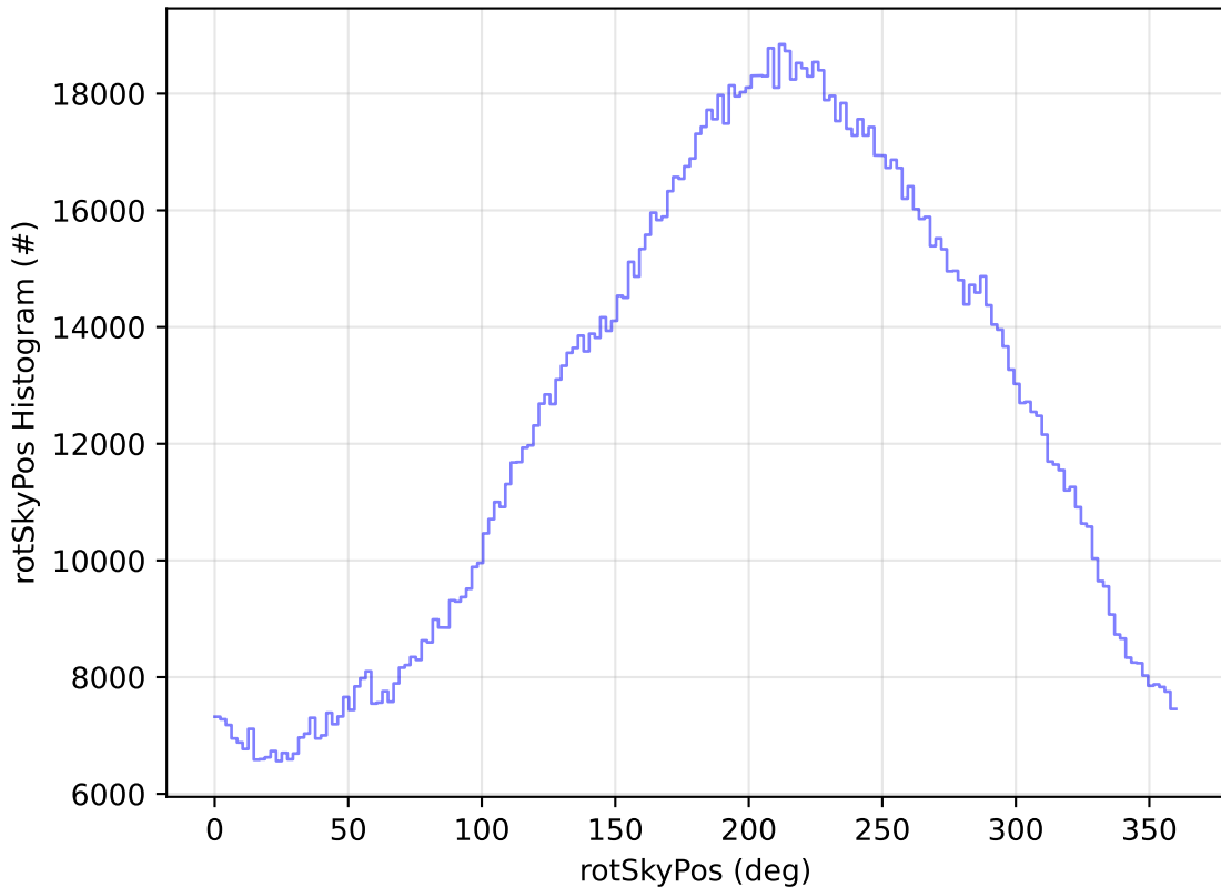
ddf_acor_sf10_lsf15_lsr10_v3.4_10yrs All sky all bands: rotSkyPos Histogram
