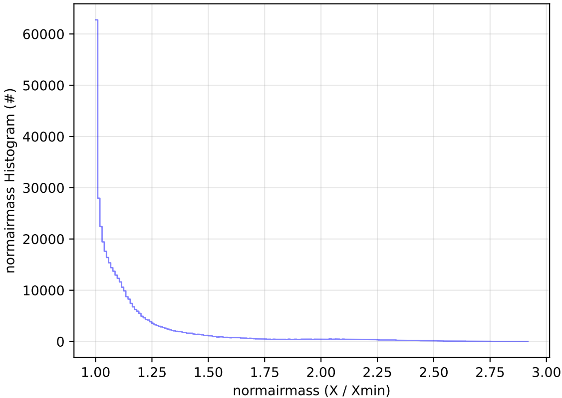
ddf_acor_sf10_lsf15_lsr10_v3.4_10yrs WFD z band: normairmass Histogram
