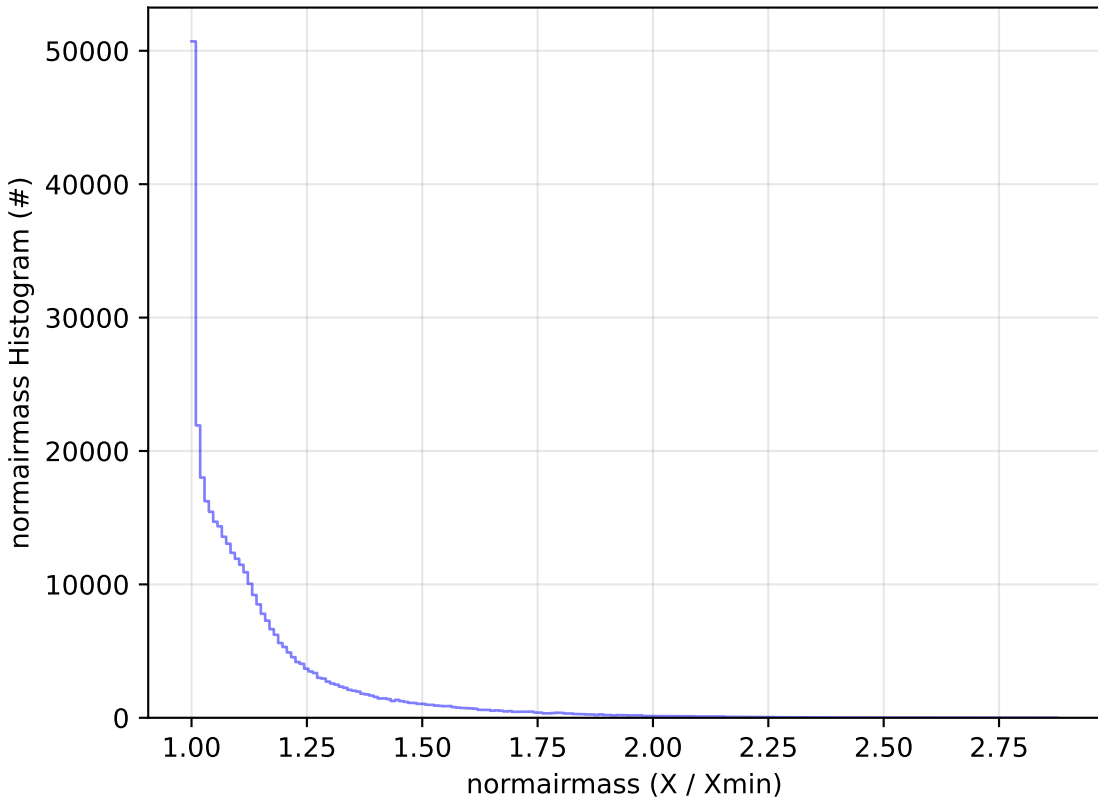
ddf_acor_sf10_lsf15_lsr10_v3.4_10yrs WFD y band: normairmass Histogram
