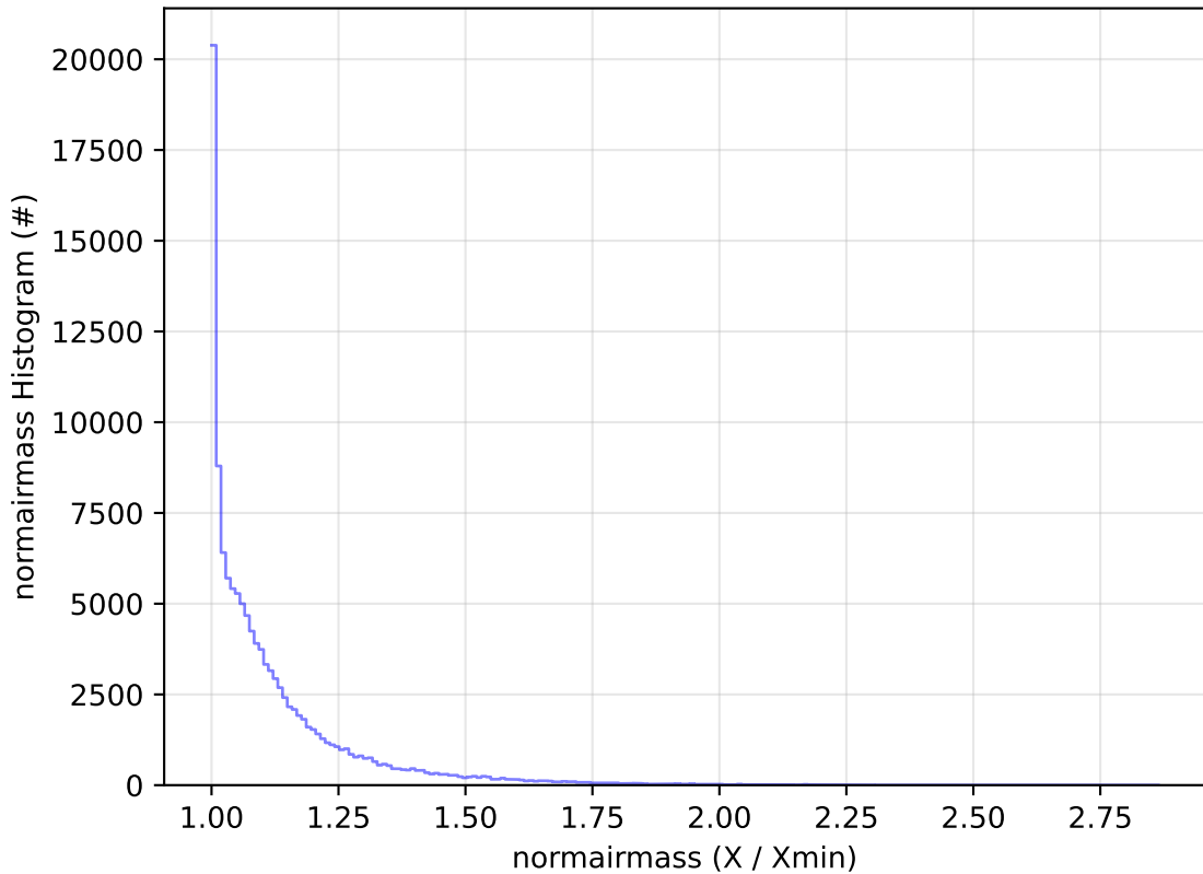
ddf_acor_sf10_lsf15_lsr10_v3.4_10yrs WFD u band: normairmass Histogram
