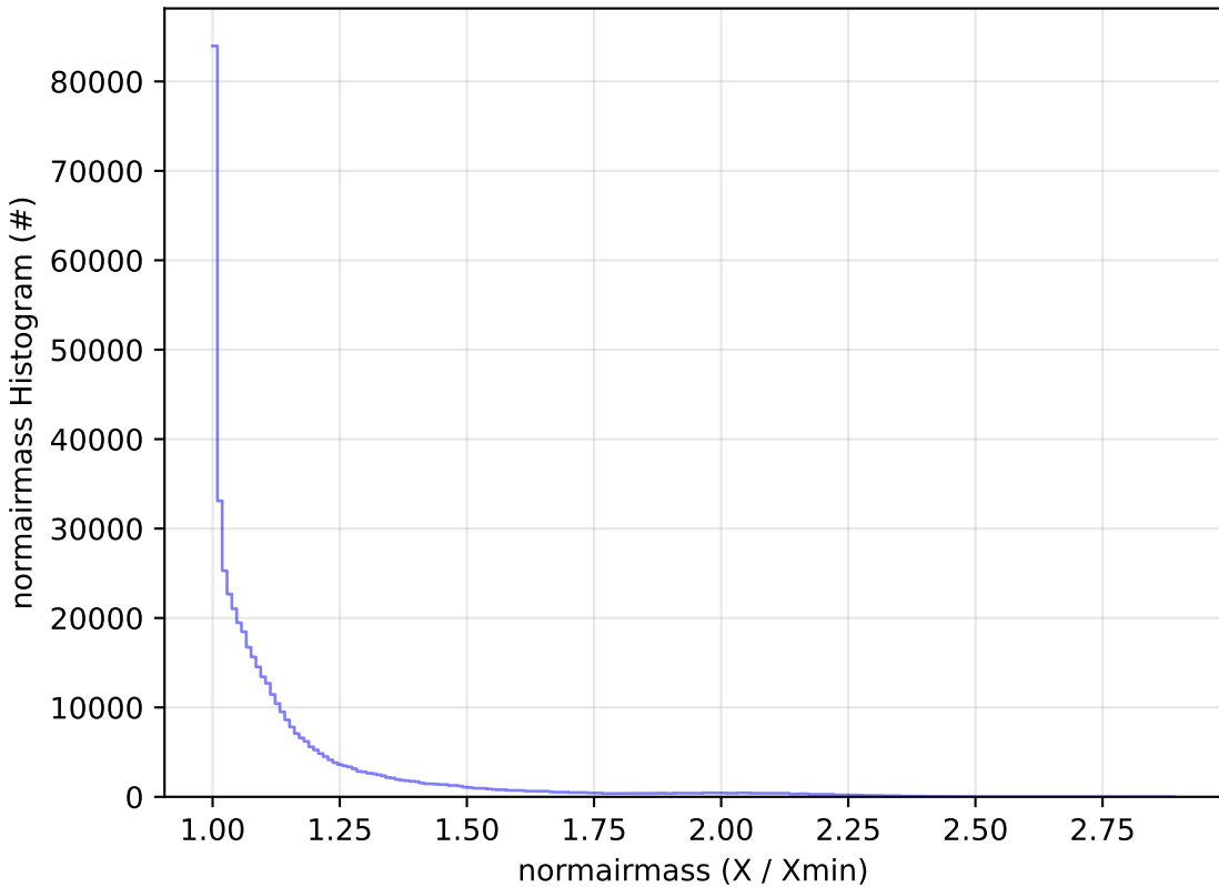
ddf_acor_sf10_lsf15_lsr10_v3.4_10yrs WFD r band: normairmass Histogram
